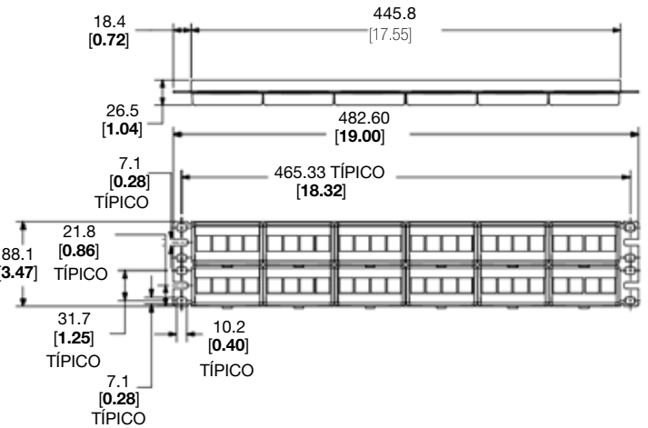
NKFPA48
