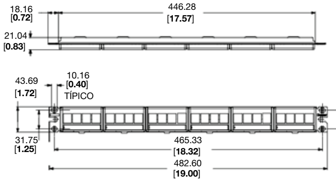
NKFP24Y
