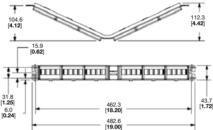
NKFPA24
