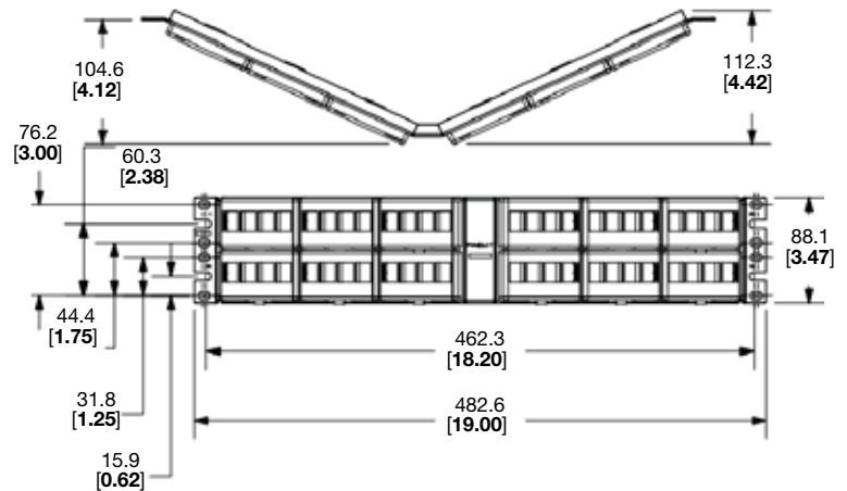
NKFPA48
